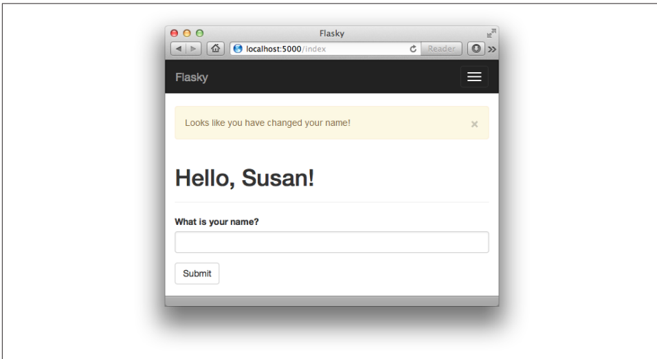
Figure 4-4. Flashed message
