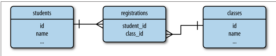
Figure 12-1. Many-to-many relationship example
